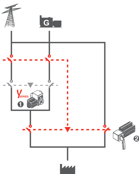
By-pass single line
