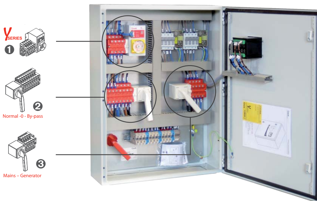
By-pass single line
